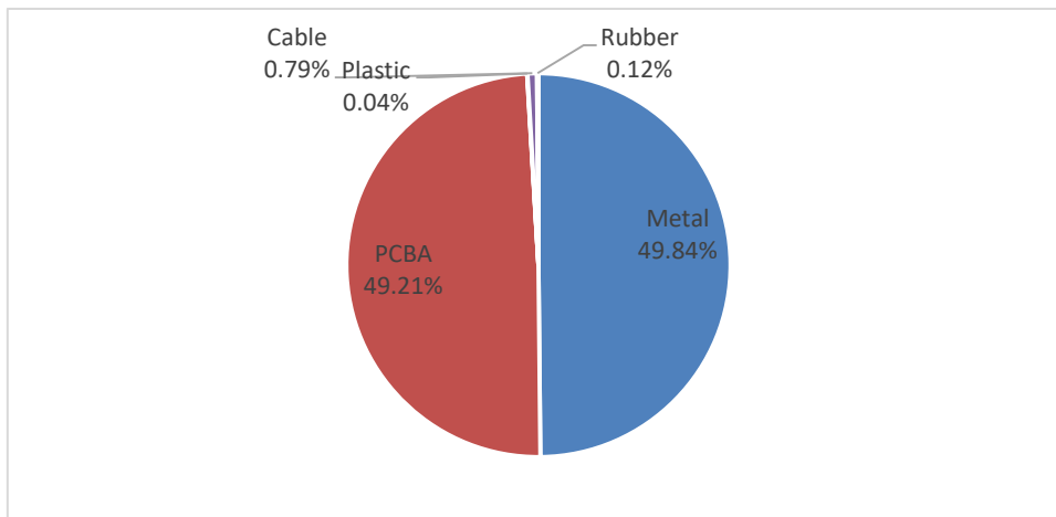
Figure 2 Main constitutive materials for SUN2000-6KTL-L1
